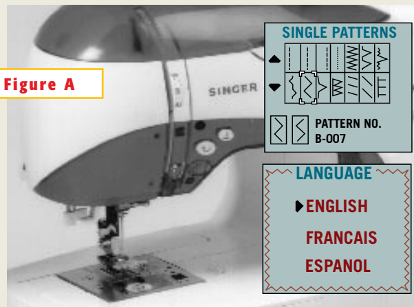
Using a Gameboy as the controller for Singer's Izek sewing machines reduces not only the cost and mechanical complexity of the stitch-programming interface, but also the time a user must spend at the sewing machine when programming stitches (top). It also allows for on-the-spot localization of control, help, and tutorial material (bottom).
